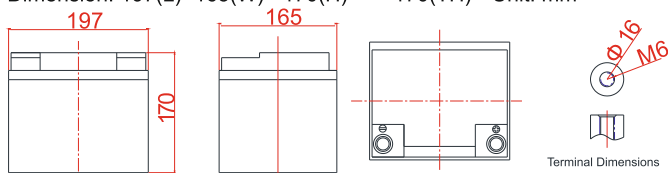
Terminal Dimensions
